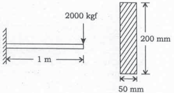
Cross-section of beam
